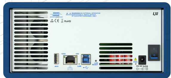
4-Slot USB/LXI Modular Chassis Front Panel
